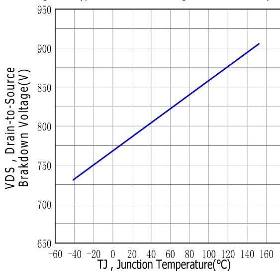
Figure.5 Typical Breakdown Voltage vs Junction Temperature
